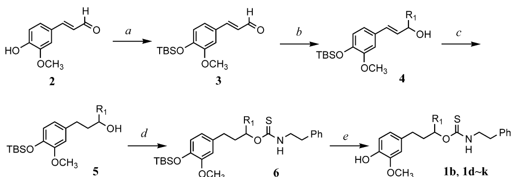
Scheme 1. Reagents and conditions: (a) NaH, THF; then TBSCl, 99%; (b) R_1\text{MgBr} , THF, 80–99%; (c) \text{H}_2 , Pd/C, MeOH, 80–100%; (d) NaH, R_2\text{NCS} , THF, 75–95%; (e) TBAF, THF, 90–99%.
