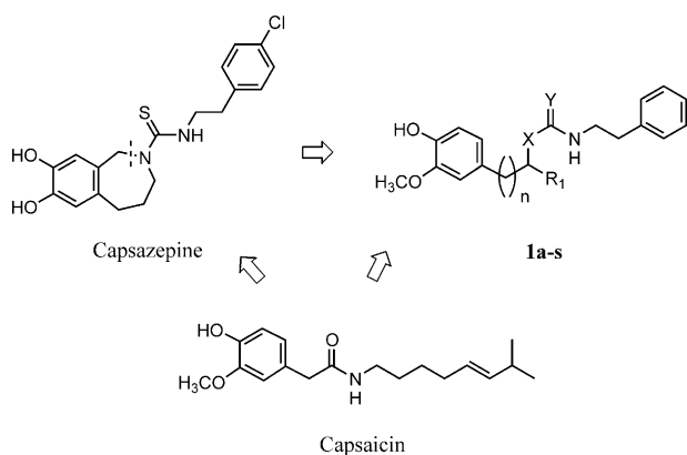
Figure 1. Structures of capsaicin, capsazepine and target molecules 1a–s .
