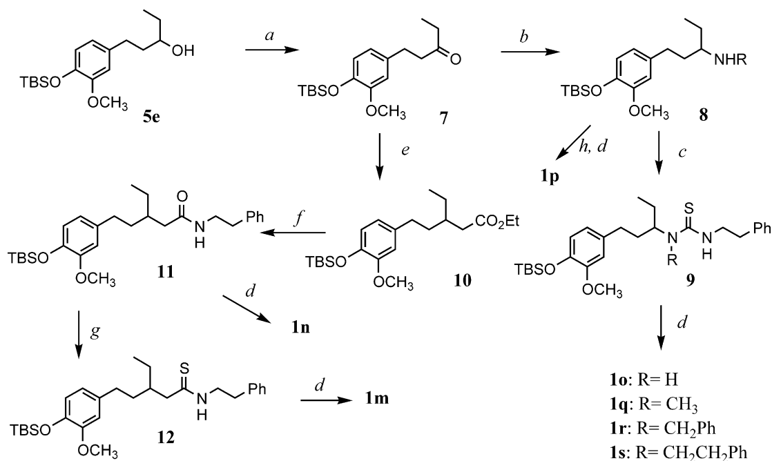
Scheme 2. Reagents and conditions: (a) PCC, CH 2 Cl 2 , 98%; (b) RNH 2 ; H 2 , Pd/C 40~85%; (c) PhCH 2 CH 2 NCS, toluene, reflux, 45~85%; (d) TBAF, THF, 75~95%; (e) (EtO) 2 POCH 2 CO 2 Et, NaH, THF, 58%; H 2 , Pd/C, 81%; (f) PhCH 2 CH 2 NH 2 , Me 3 Al, CH 2 Cl 2 , 98%; (g) Lawesson's reagent, toluene, 80 °C, 47%; (h) phenethylamine, diethyl dicarbonate, DMAP, CH 2 Cl 2 , 21%.
